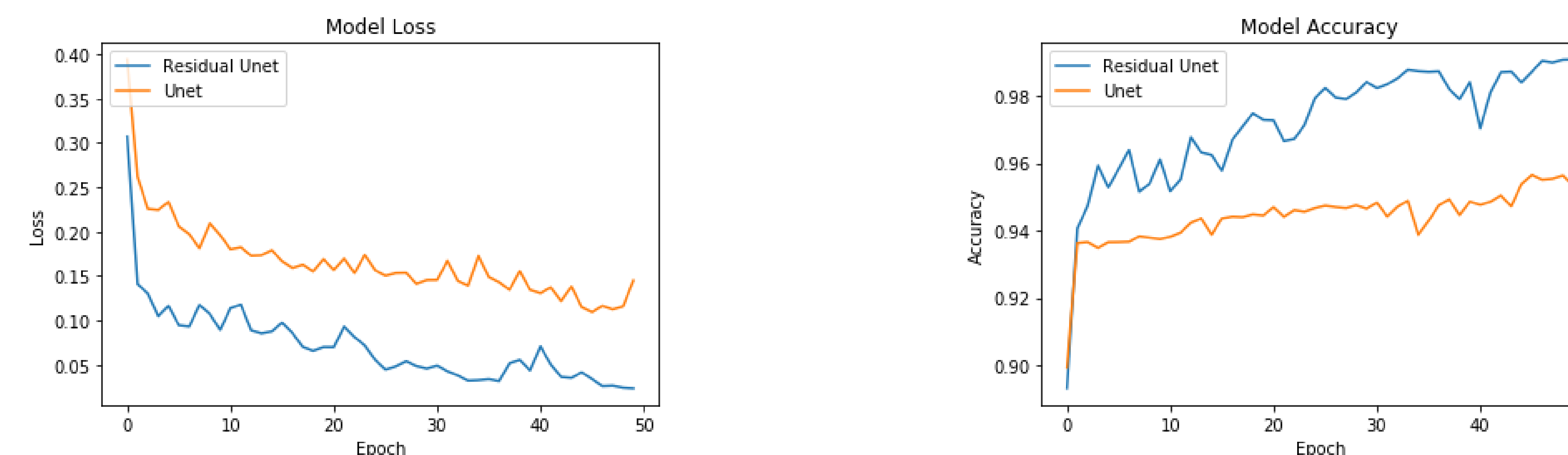
Figure 2: The loss and accuracy of U-Net and Residual U-Net models on the training set.
