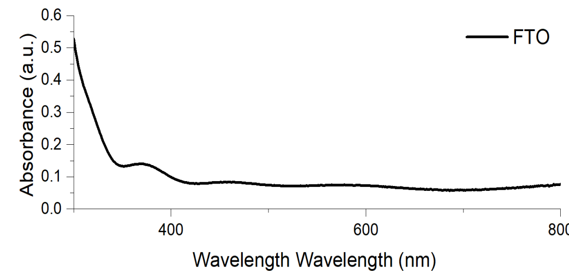
Figure 3 Absorbance spectrum graph of FTO glass
